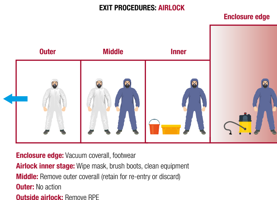
Figure 9.4 Preliminary decontamination procedures (on exiting the enclosure (from right to left))
